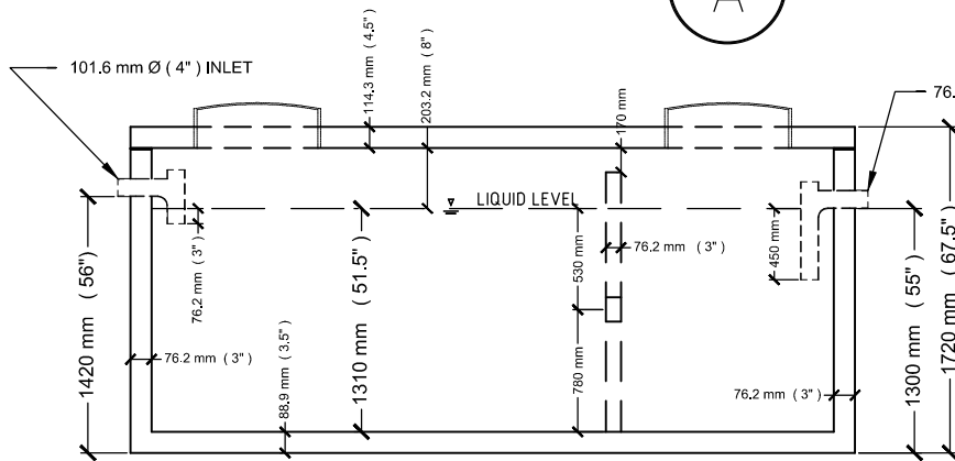
CROSS SECTION A
